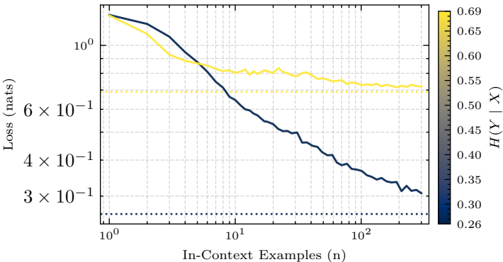
In-Context Learning Loss for Qwen-2.5 (0.5B)
